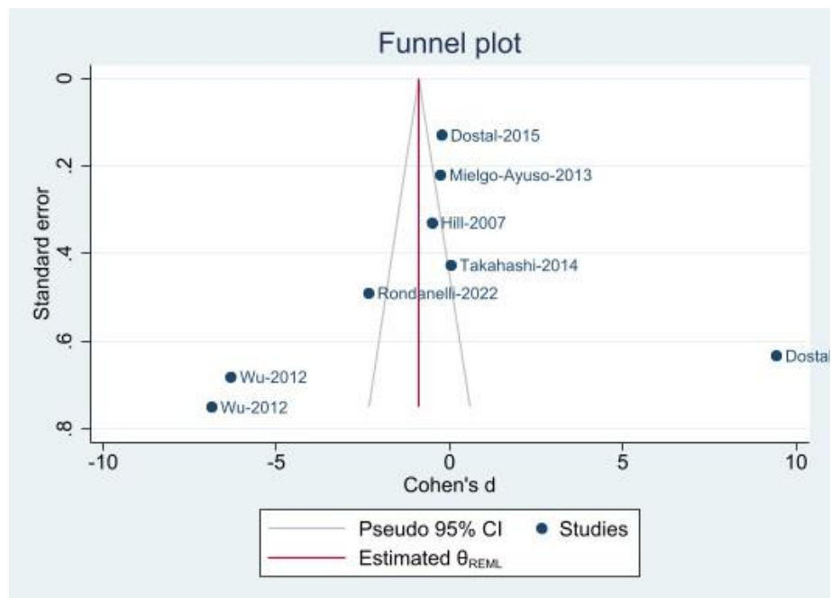
Figure 4. Funnel plot for publication bias of Insulin
