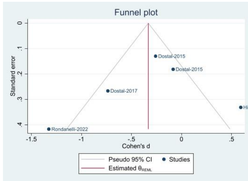
Figure 1. Funnel plot for publication bias of Leptin
