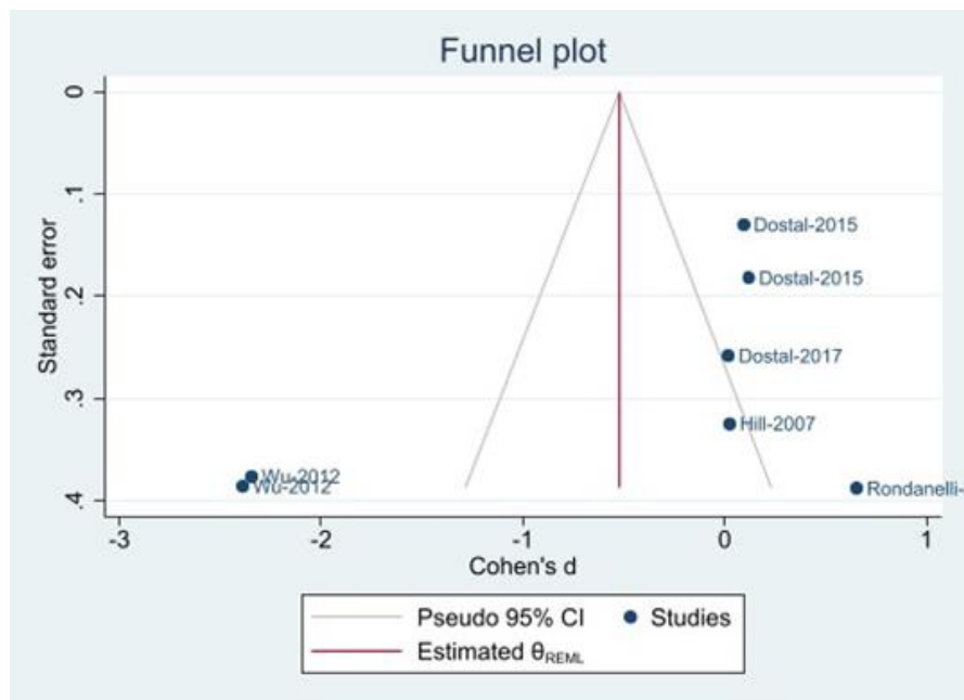
Figure 2. Funnel plot for publication bias of Adiponectin
