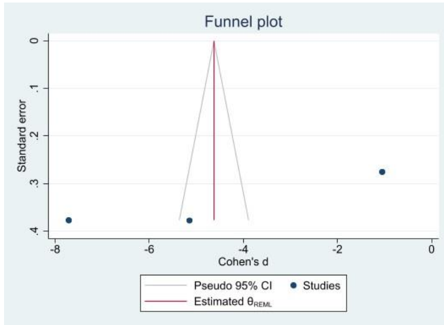
Figure 3. Funnel plot for publication bias of Ghrelin
