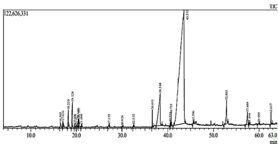
Figure 1. GC-MS complete chromatogram of Prunus amygdalus oil
